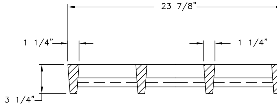
GRATE SECTION
